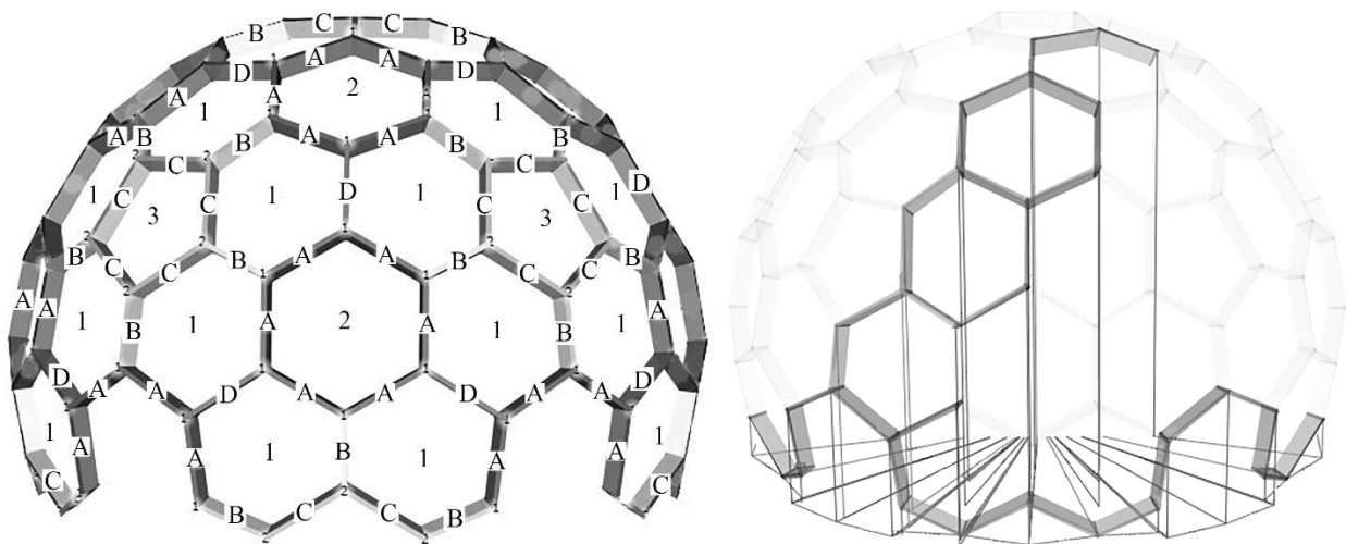
Fig. 3. Geodome frame
